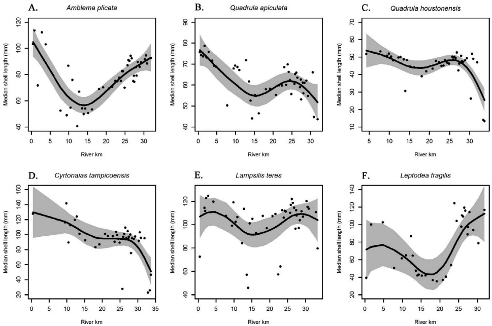
FIG. 3.—General additive models (GAM) of median shell length (mm) and the distance (river-km) of study sites downstream from Lake Somerville in Yegua Creek, Texas. Models are for the 6 most abundant species in Yegua Creek: (A) Amblema plicata , (B) Quadrula apiculata , (C) Quadrula houstonensis , (D) Cyrtoniais tampicoensis , (E) Lampsilis teres and (F) Leptodea fragilis . Shaded areas indicate 95% confidence intervals
