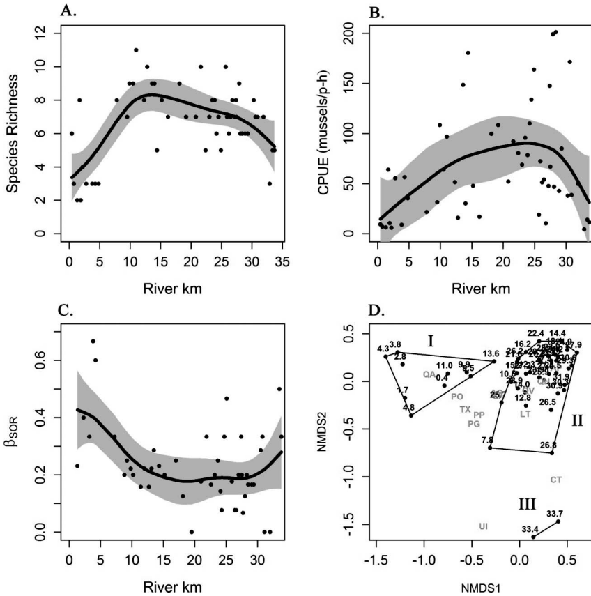
FIG. 2.—(A) General additive models (GAM) representing the relationship between species richness (number of species), (B) catch-per-unit-effort (CPUE; mussels/person-hours of search effort), and (C) beta diversity ( \beta_{SOR} ) of mussels with the distance (river-km) of study sites downstream from Lake Somerville in Yegua Creek, Texas. Shaded areas indicate 95% confidence intervals. (D) NMDS biplot of mussel assemblage structure ( S = 0.10 , k = 2 ). Sites and species are represented by black points and species abbreviations (red text; Table 1), respectively. Lines connecting site clusters were derived from the agglomerative cluster analysis. Mussel assemblages in lower Yegua Creek are labeled the following: (I) reservoir-influenced (lentic), (II) lotic, and (III) Brazos River assemblages
